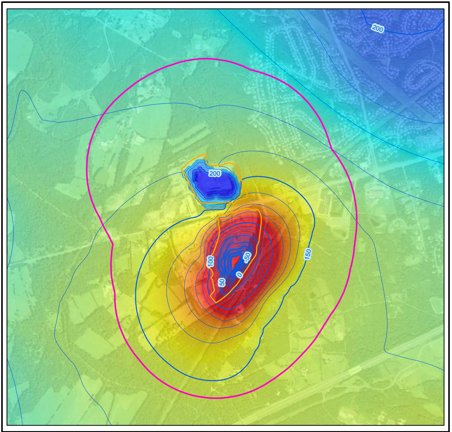
Figure 4i: Model-Predicted Groundwater Elevations at Fill Sequence 5
