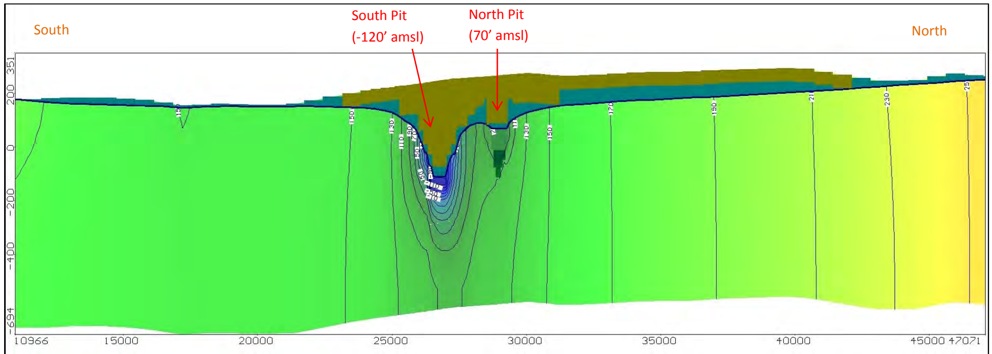
Figure 4d: Fill sequence 2 cross-sectional view of groundwater elevations sliced through the Fairfax Quarry's North Pit and South Pit. Bronze-colored areas represent dry model grid cells. Contour interval = 20 feet. X-axis labels are in units of feet and Y-axis labels are in units of feet above mean sea level. Vertical exaggeration = 10x.
