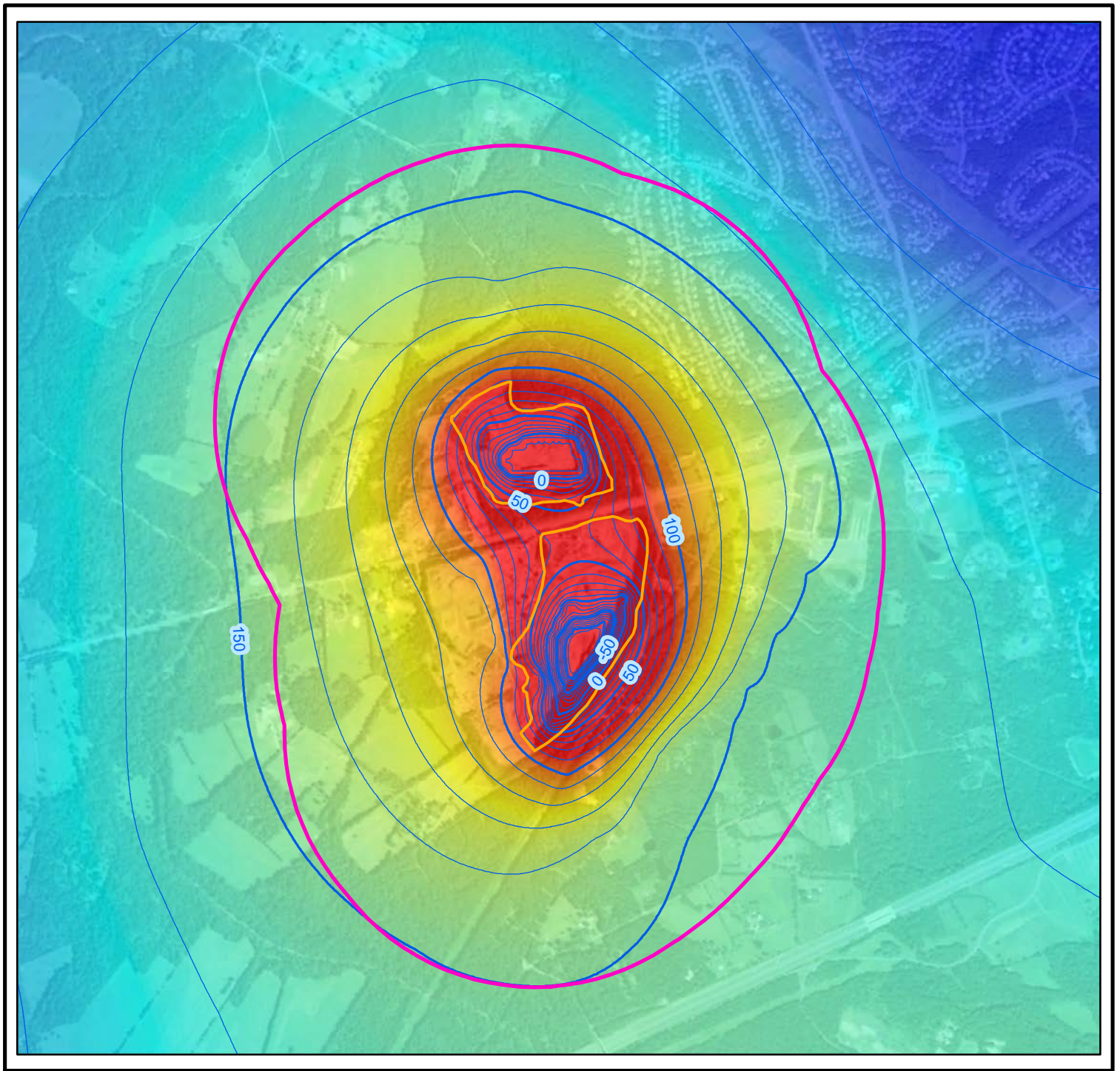
Figure 4a: Model-Predicted Groundwater Elevations at Fill Sequence 1
