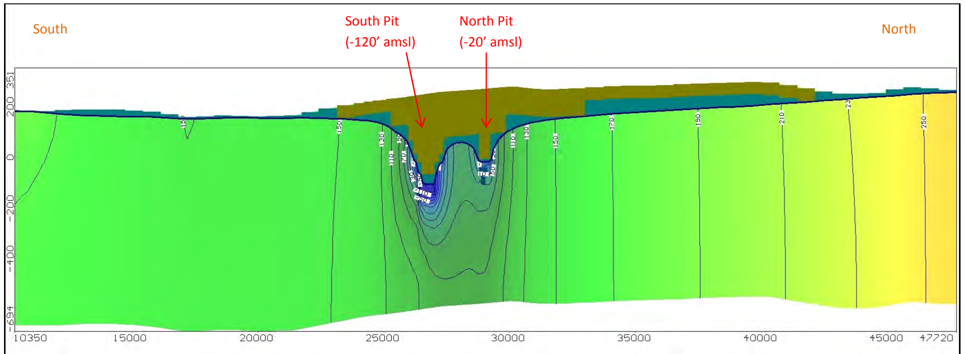
Figure 4b: Fill sequence 1 cross-sectional view of groundwater elevations sliced through the Fairfax Quarry's North Pit and South Pit. Bronze-colored areas represent dry model grid cells. Contour interval = 20 feet. X-axis labels are in units of feet and Y-axis labels are in units of feet above mean sea level. Vertical exaggeration = 10x.
