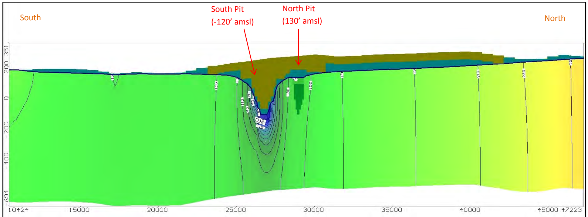
Figure 4f: Fill sequence 3 cross-sectional view of groundwater elevations sliced through the Fairfax Quarry's North Pit and South Pit. Bronze-colored areas represent dry model grid cells. Contour interval = 20 feet. X-axis labels are in units of feet and Y-axis labels are in units of feet above mean sea level. Vertical exaggeration = 10x.
