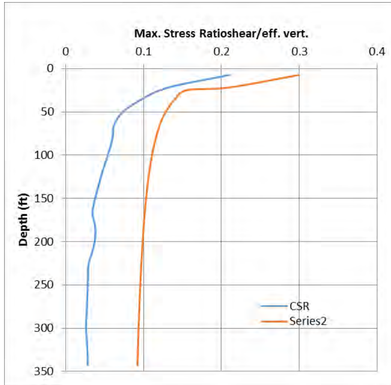
CSR for Mineral Virginia at Reston vs. CRR
