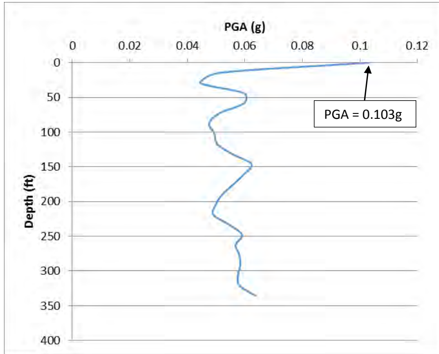
PGA vs. Depth for Mineral, VA Ground Motion Measured at Reston, VA for the stiff profile
