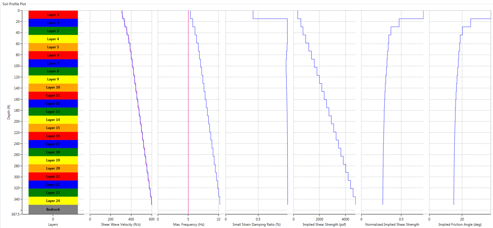
Input Firm Soil Profile for Site Response Analysis
