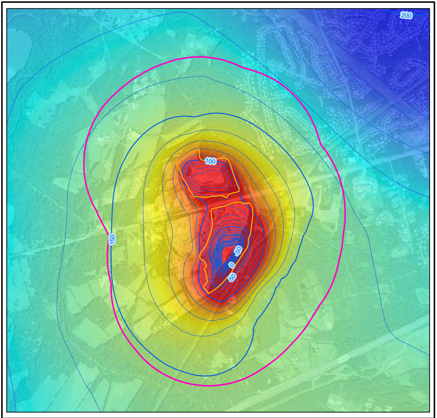
Figure 4c: Model-Predicted Groundwater Elevations at Fill Sequence 2
