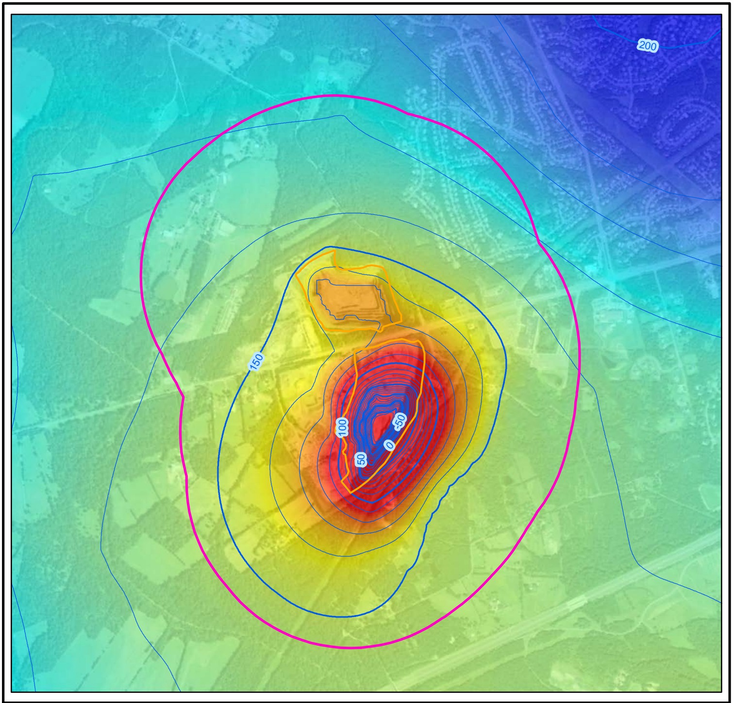
Figure 4e: Model-Predicted Groundwater Elevations at Fill Sequence 3
