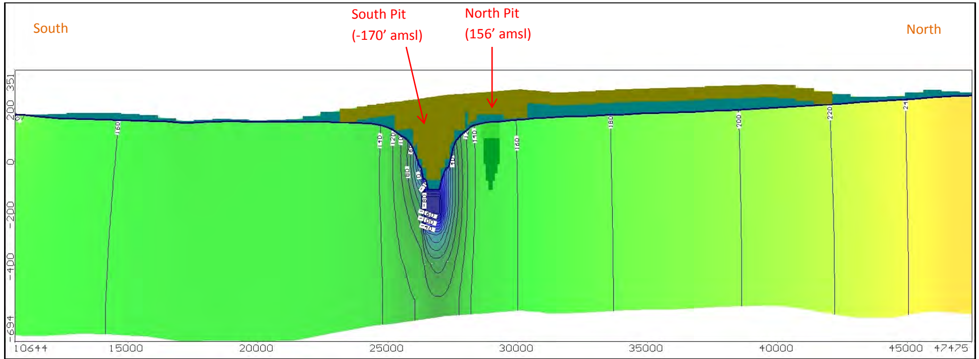
Figure 4h: Fill sequence 4 cross-sectional view of groundwater elevations sliced through the Fairfax Quarry's North Pit and South Pit. Bronze-colored areas represent dry model grid cells. Contour interval = 20 feet. X-axis labels are in units of feet and Y-axis labels are in units of feet above mean sea level. Vertical exaggeration = 10x.
