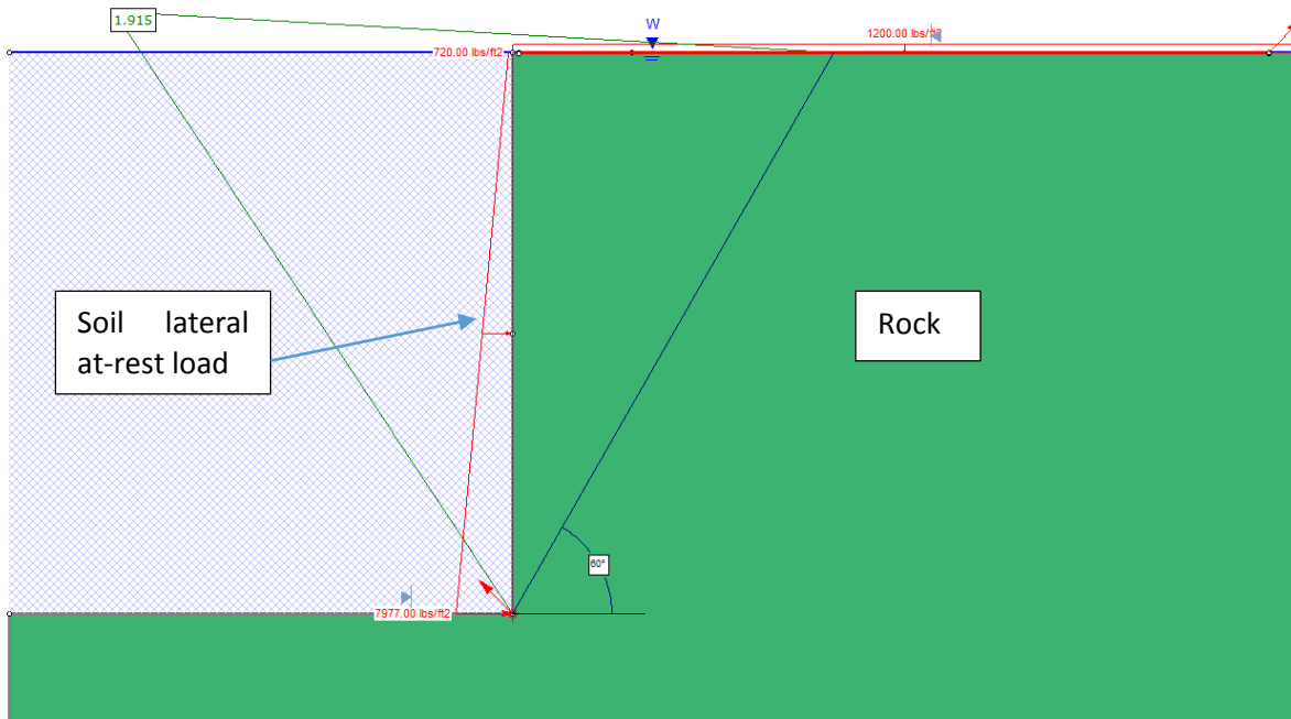
Limit Equilibrium Soil Model with Resulting Minimum Factor of Safety
