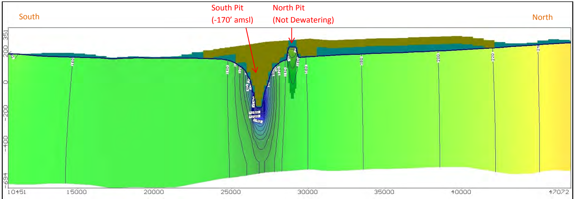
Figure 4j: Fill sequence 5 cross-sectional view of groundwater elevations sliced through the Fairfax Quarry's North Pit and South Pit. Bronze-colored areas represent dry model grid cells. Contour interval = 20 feet. X-axis labels are in units of feet and Y-axis labels are in units of feet above mean sea level. Vertical exaggeration = 10x.
