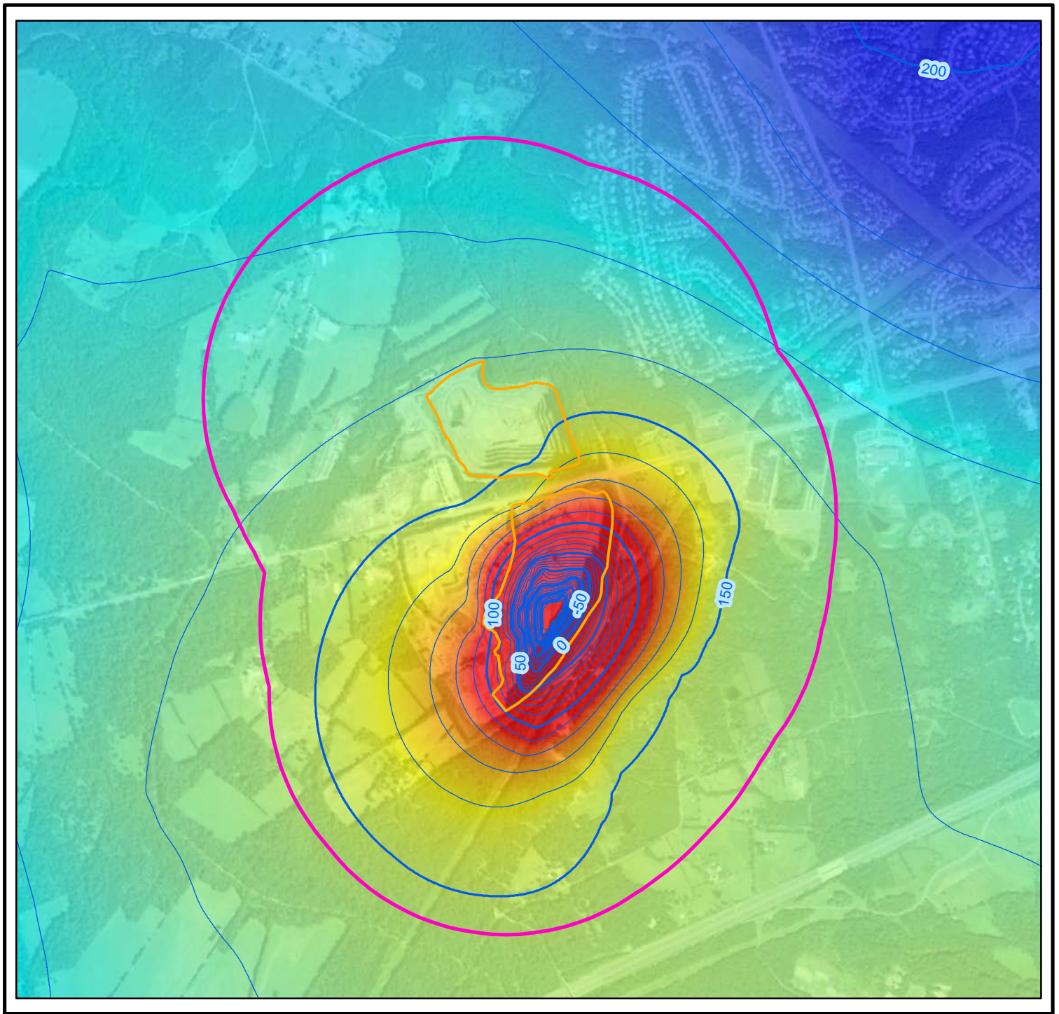
Figure 4g: Model-Predicted Groundwater Elevations at Fill Sequence 4
