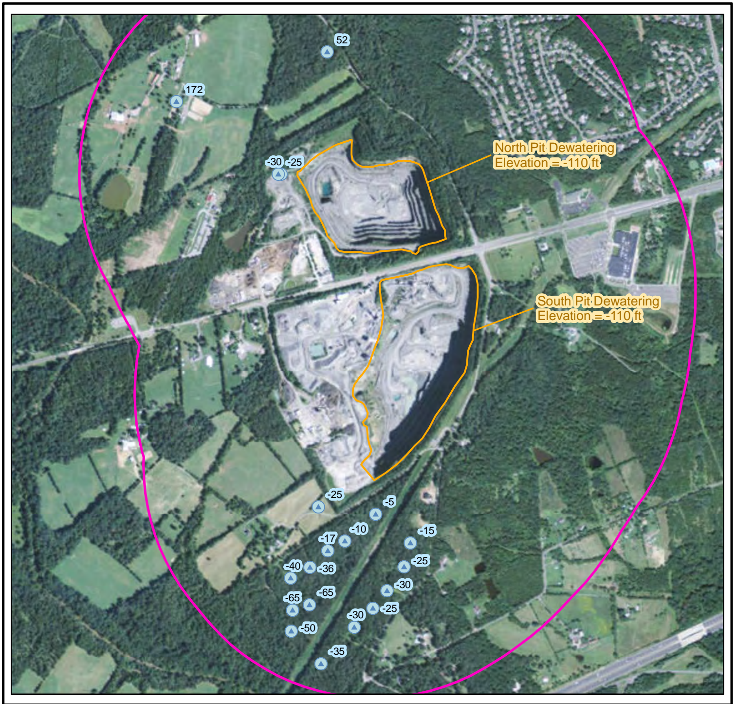
Figure 3: Estimated Groundwater Elevations in Proximity to the Quarry
